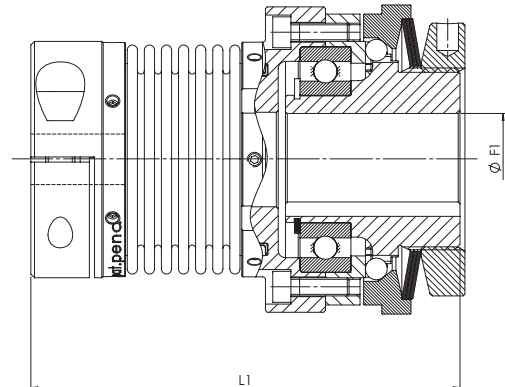
Bore and keyway execution / GSP
