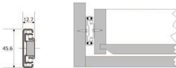
Installation Diagram
