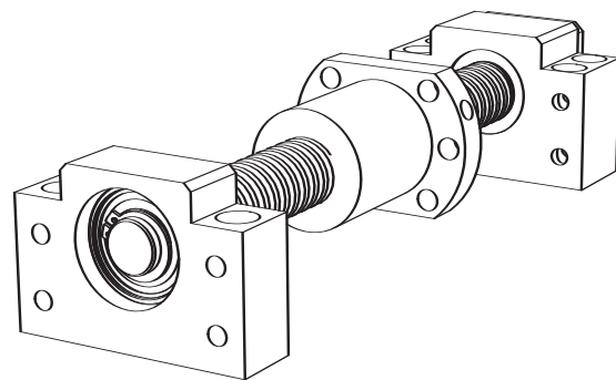
Supported end
